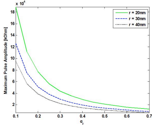
Fig. 6 Maximum pulse amplitude versus \alpha_r for 3 written mark-radiuses.
