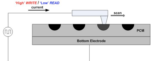
Fig. 1 Scanning-probe system architecture.
