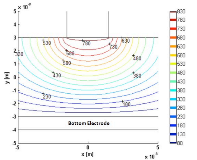
Fig. 3 Isothermal contours showing the temperature distribution throughout the GST layer, after the application of a voltage pulse with amplitude 0.5-V for 45 nsec.
