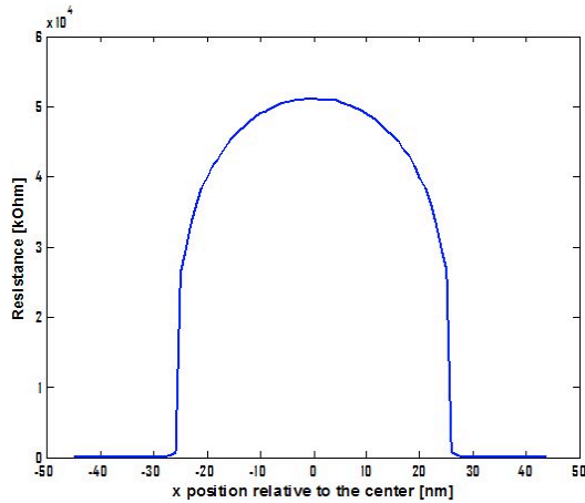
Fig. 5 A typical read-back pulse obtained by reading a single amorphous mark with radius r=30nm .
