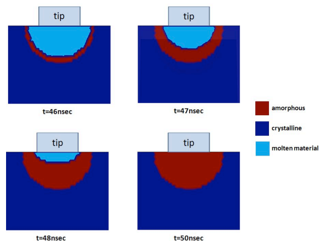
Fig. 4 Spatial distribution of amorphization during cooling process.
